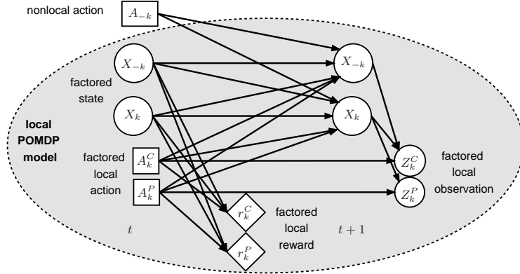
Fig. 2. The factored decision model, from agent k 's perspective.
