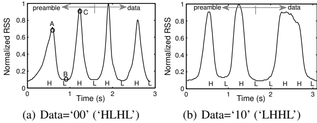
Figure 5: Received signals in an ideal scenario.
