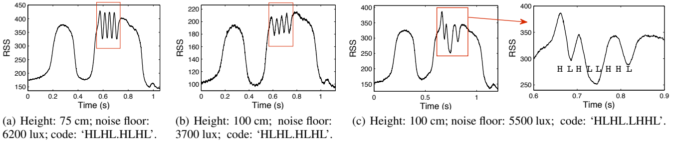
Figure 17: Car's speed is 18 km/h. Two different types of code and different distance between the car and the receiver.
