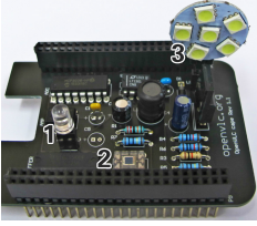
Figure 3: The evaluation board runs a Debian Linux and the open-source OpenVLC driver. We receive data using either the low-power LED (1) or the photodiode (PD) (2). Key used electronic devices are listed on the right.
