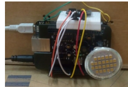
Figure 9: Sensors connected through serial to the BBB, and the BBB to the computer via USB
