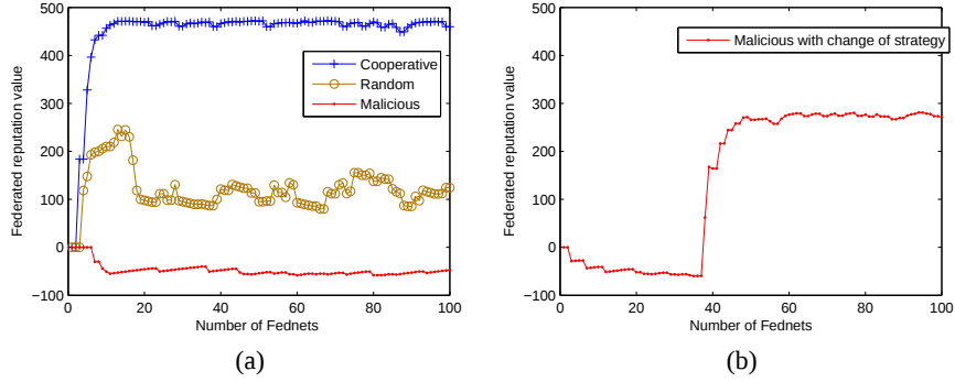
Figure 19.6: Building federated reputation based on the strategy.
