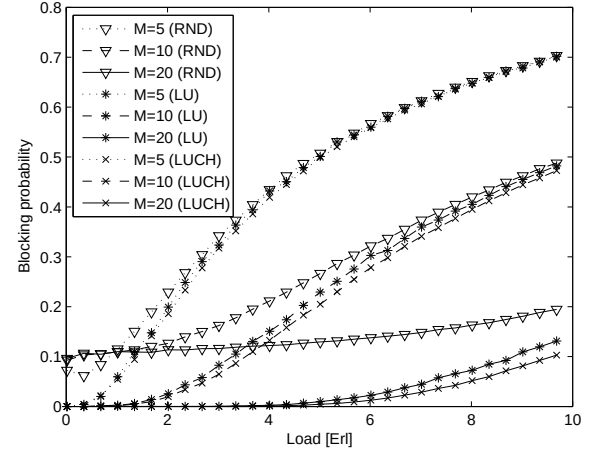
Fig. 4. Simulation of blocking probability for M=\{5,10,20\} for different channel access schemes. Channels are utilized non-uniformly by PUs, i.e., for m = 1, \dots, M/2, \forall m > 2, \lambda_{p,m} = \lambda_{p,m-1} - \lambda_{p,1}/2, \lambda_{p,1} = 20 and \mu_{p,M} = 3 . Rest of the channels are considered unoccupied by PUs.
