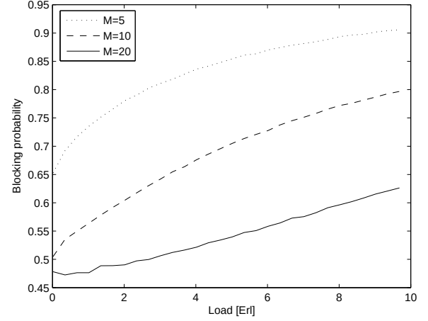
Fig. 3. Simulation of blocking probability for M=\{5,10,20\} where DSAN was using RND algorithm. Channels are utilized non-uniformly by PUs, i.e., \forall m > 2, \lambda_{p,m} = \lambda_{p,m-1} - \lambda_{p,1}/2, \lambda_{p,1} = 20 and \mu_{p,M} = 3 .
