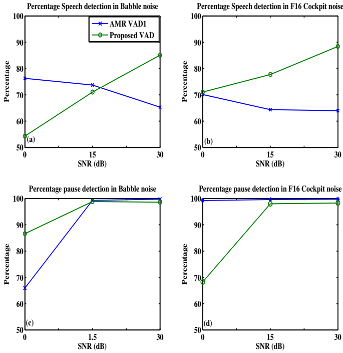
Fig. 3. Performance comparison between AMR VAD1 and the proposed method. (a) and (b) Percentage speech detection performance under Babble and F16 Cockpit noise conditions (c) and (d) Percentage pause detection under Babble and F16 Cockpit noisy conditions. SNR is varied from 0 to 30 dB.
