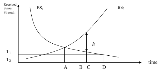
Fig. 12. Received signal strength when MS travels in the handoff area
