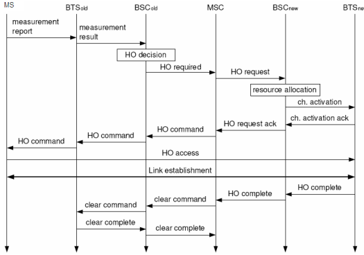
Fig. 6. Intra-MS handoff in GSM
