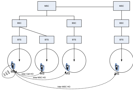
Fig. 5. Handoff types in GSM
