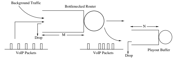
Fig. 2. VoIP session simulation model; M , N - queue size of bottleneck router and playout buffer, respectively.
