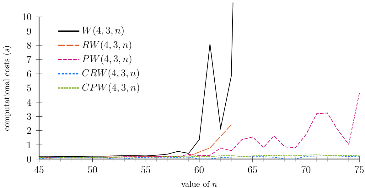
Figure 5: Costs to compute W(4, 3, n) by using some forced patterns.
