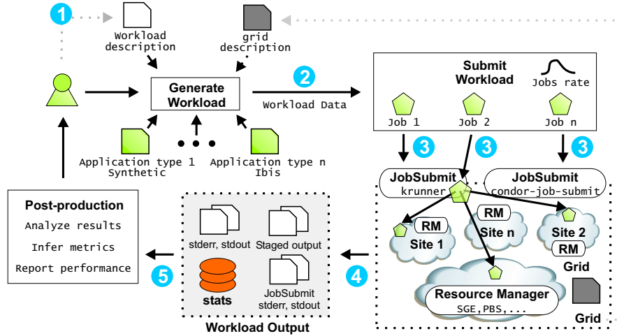
Figure 1. The GRENCHMARK process.
