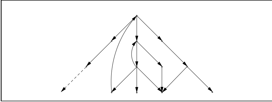
Fig. 4. Phenomena in composition of transformation rules: infinite branches, inverses, confluence, non-confluence
