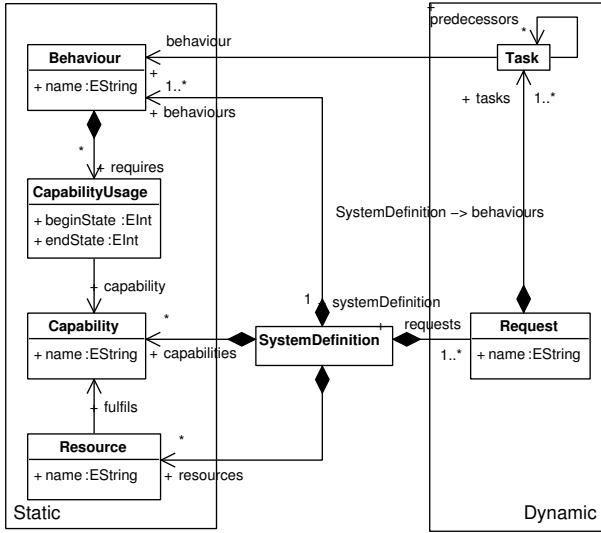
Figure 6: Target metamodel
