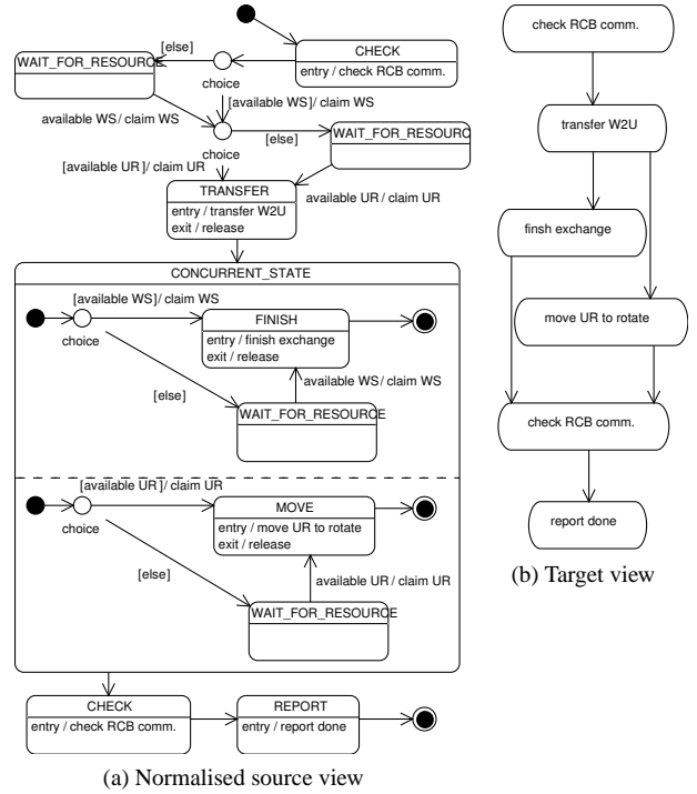
Figure 7: Unload wafer request transformation
