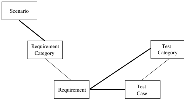
Figure 2. Traceability Meta-Model
