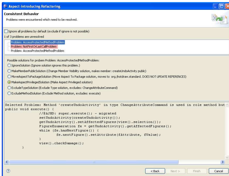
Fig. 9 Challenge resolution in SAIR.
