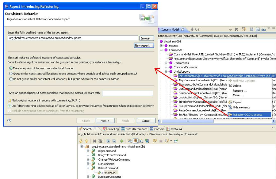
Fig. 8 SAIR's integration with SOQUET and user interface for input collection.
